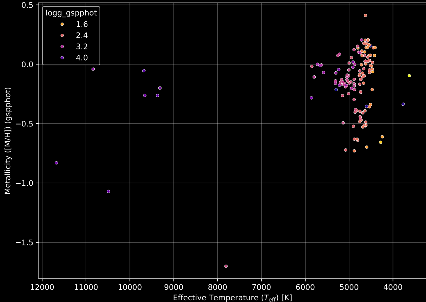
APOGEE DR17 Field: [Per_M_MGA] Stellar Population Parameters (n= 147)
