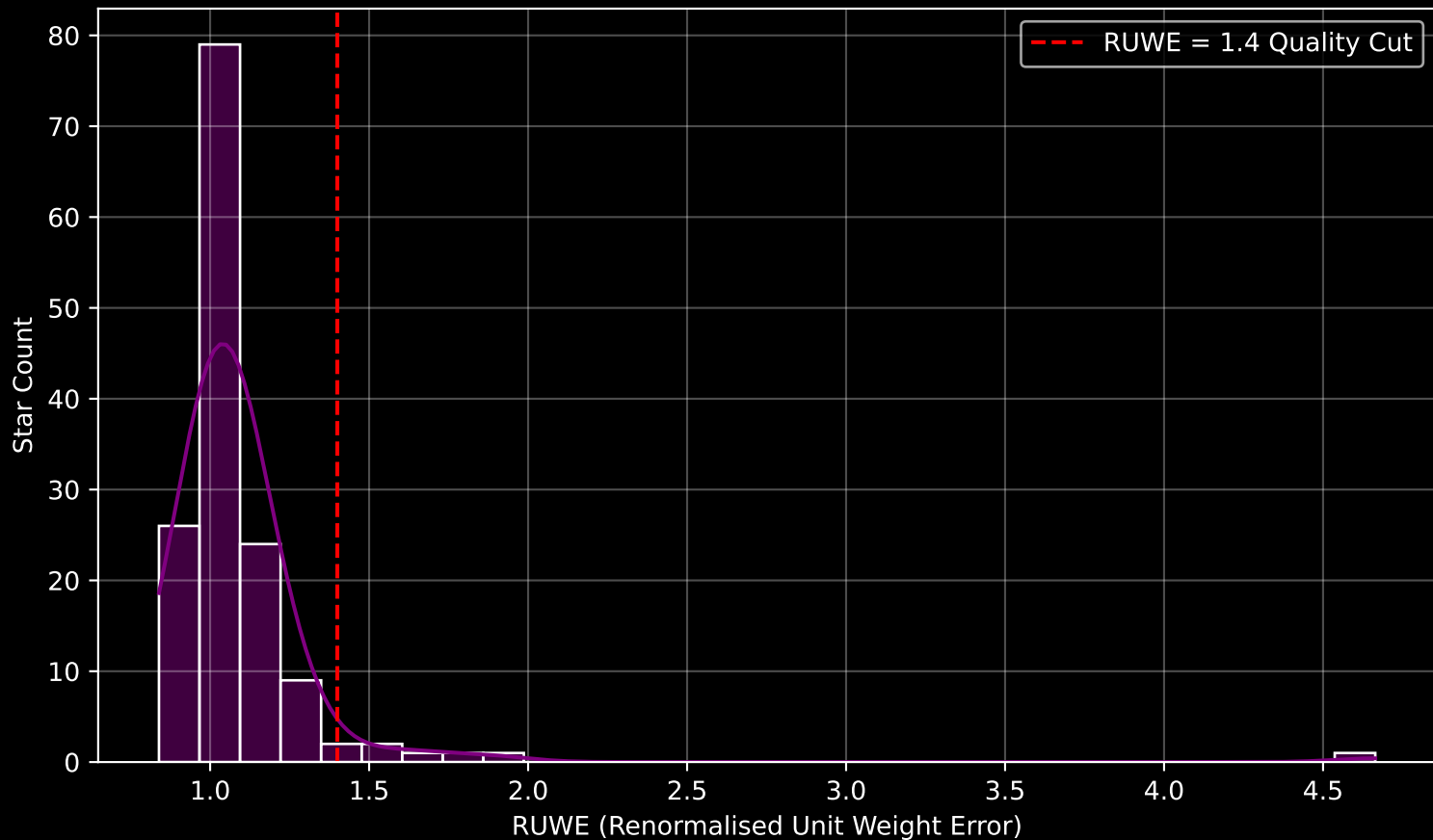
GAPOGEE DR17 Field [Per_M_MGA] RUWE Distribution (n= 146)
