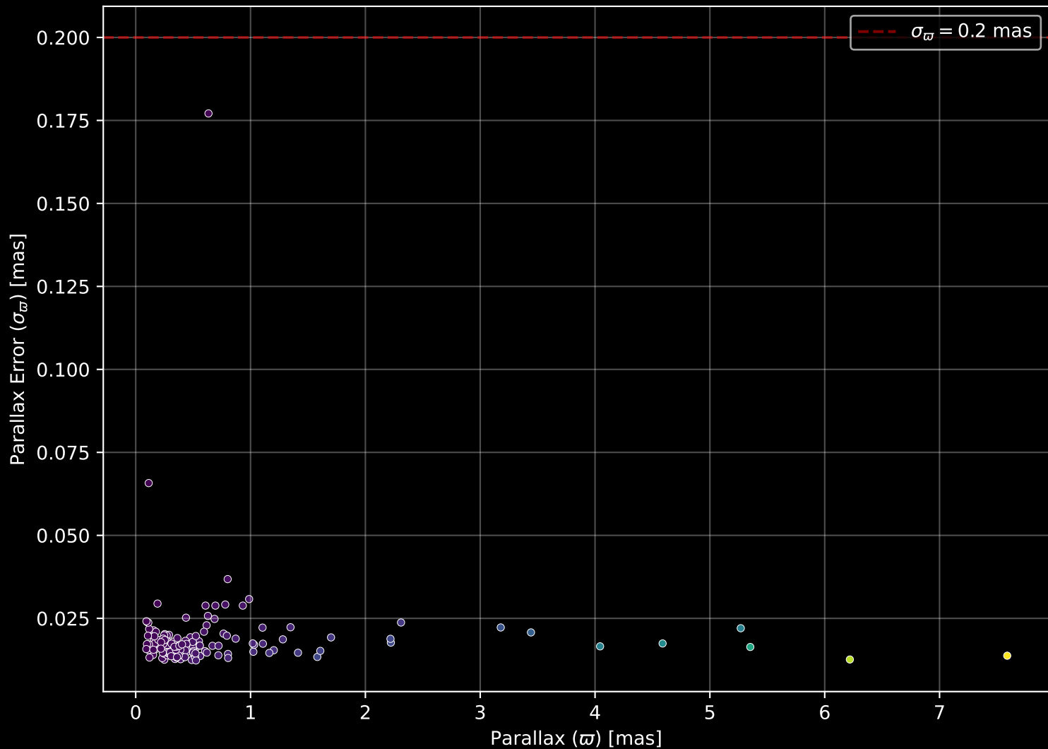
APOGEE DR17 Field: [Per_M_MGA] Parallax Quality (n= 147)
