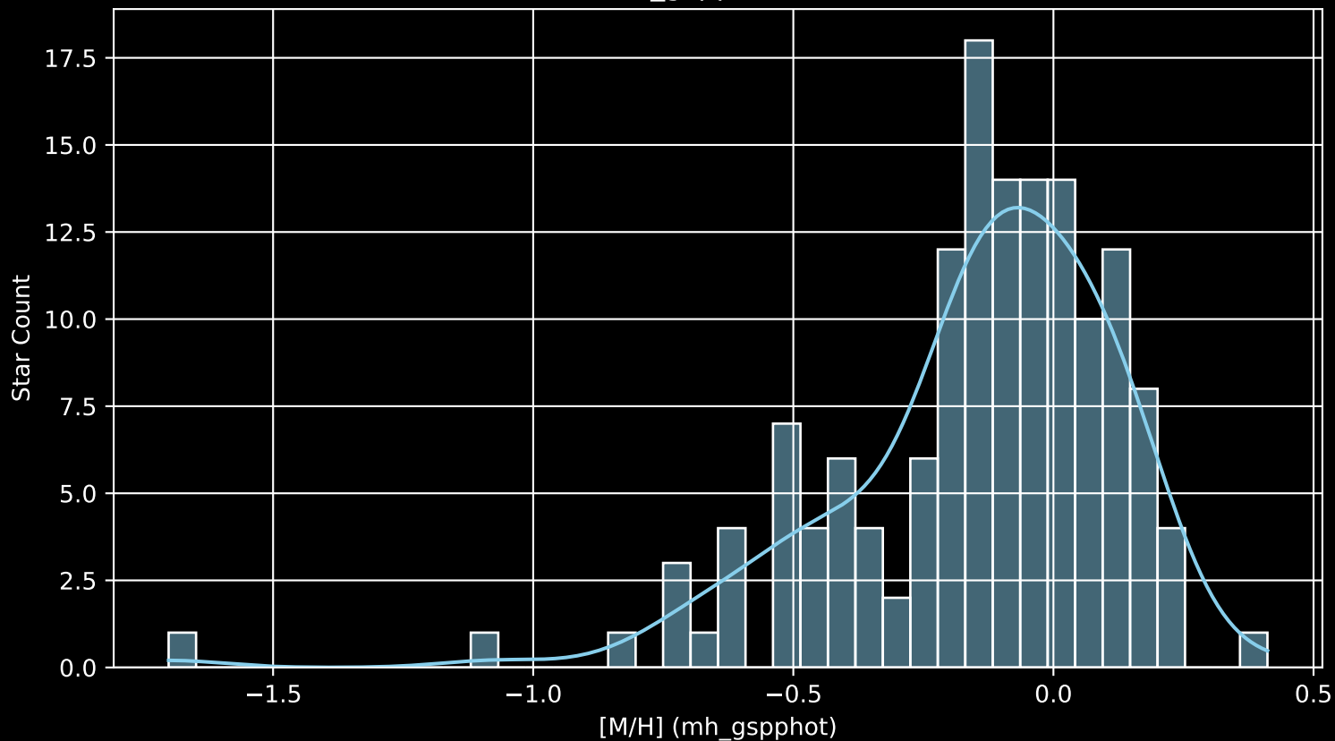
APOGEE DR17 Field: [Per_M_MGA [M/H] (mh_gspphot) (n= 147)
