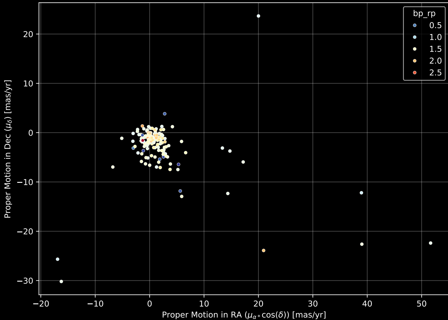
APOGEE DR17 Field: [Per_M_MGA] Proper Motion Diagram (n= 147)
